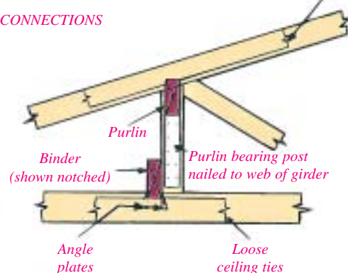
Loose rafters notched onto purlin
