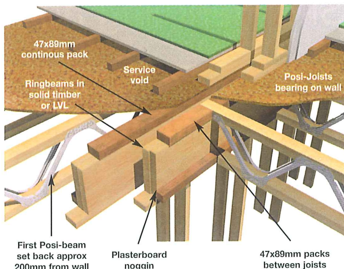
Timber frame party wall (with service void)
