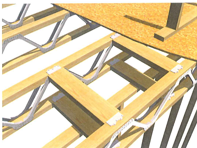
Non-load bearing partitions parallel to floor beams
