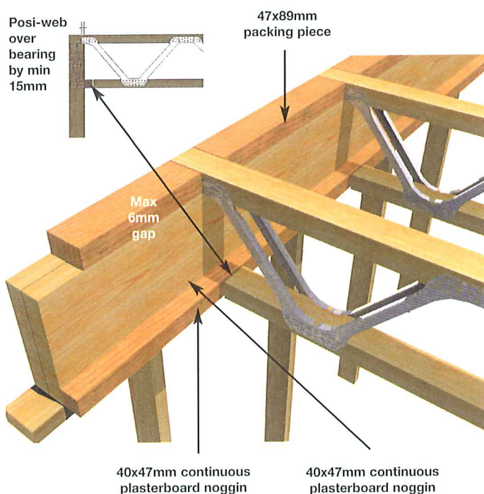
Non-load bearing partitions parallel to floor beams
